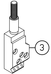
Needle Clamp(5.6)
